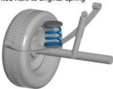
Auxiliary Coil Spring HV-.....0 mounted next to original spring
